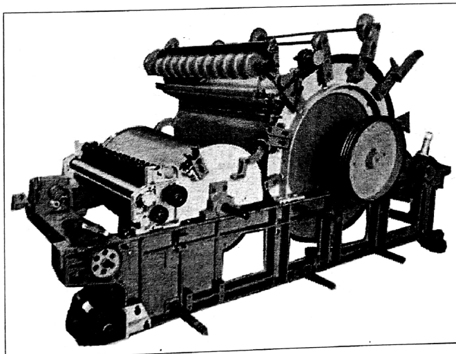
Fig 6: Hand carding machine
